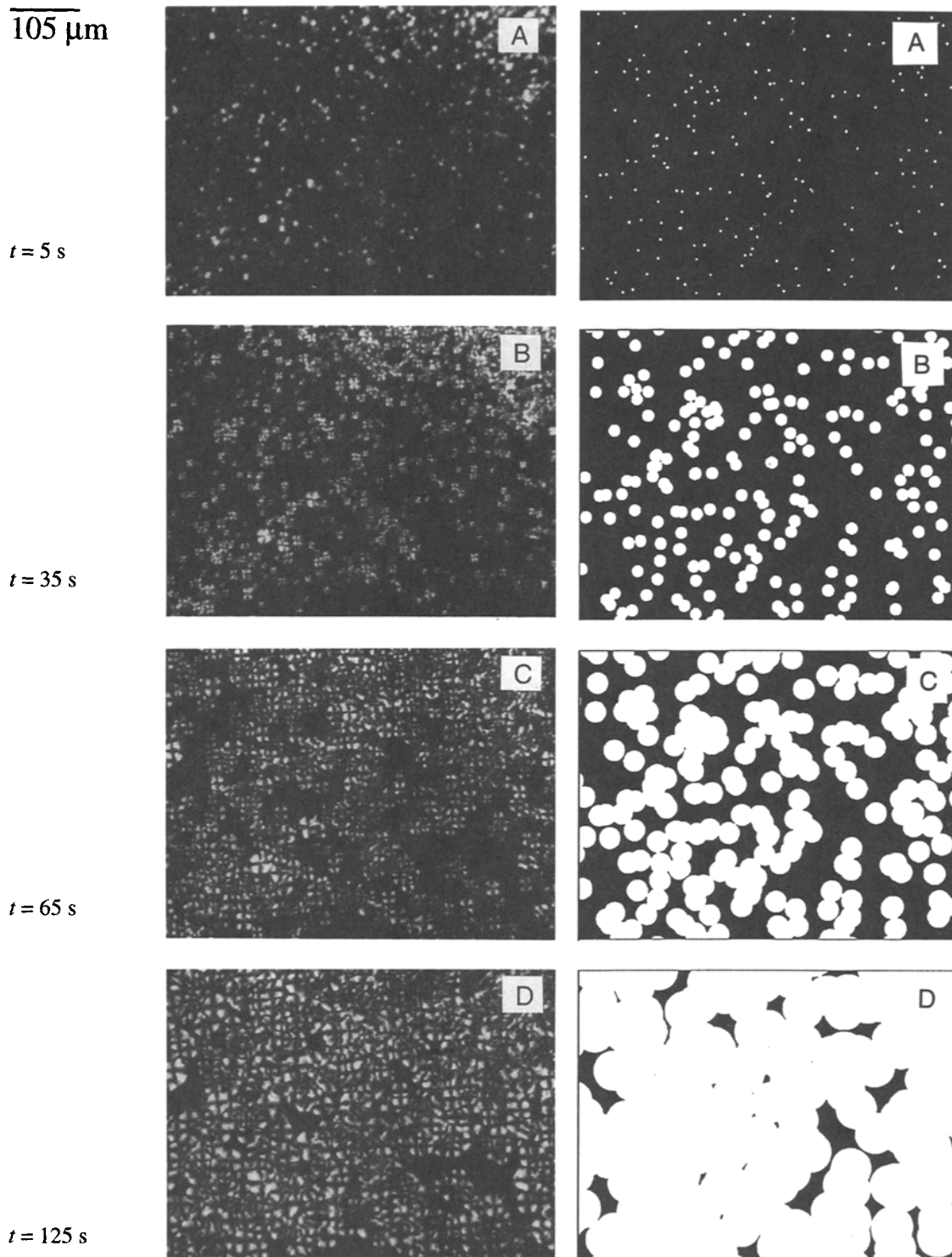
FIG. 7. Experimental (left) and simulated (right) polarized light microscopy views of a POP sample solidifying at 15°C, at different times. Abbreviations as in Figures 1 and 2.
